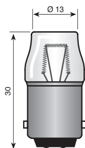
Ba15d
