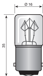
Ba15d
