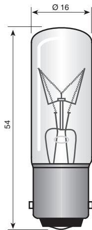
Ba15d
