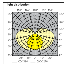
LS LED 1200 20.5W
