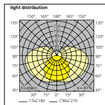
LS LED 900 15.3W
