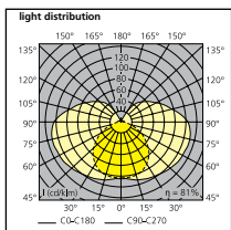
LS LED 600 10.2W
